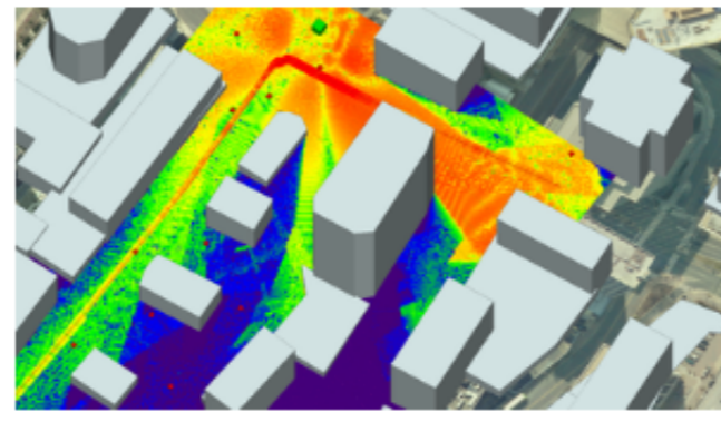
Beamforming Simulations
